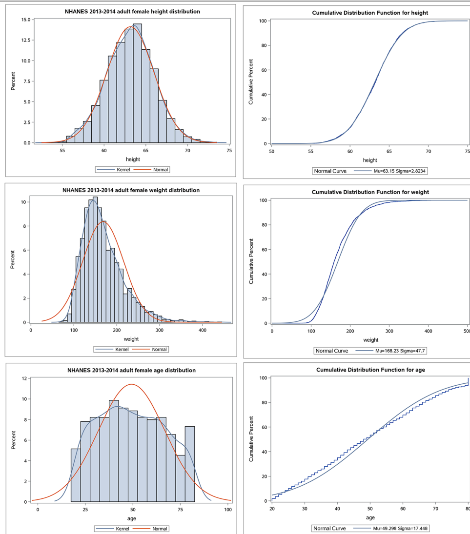
Figure 8.8: NHANES 2013–2014 height, weight, and age distributions for females
