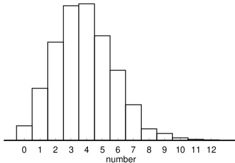
Figure 7.8: Histogram for radioactive disintegrations (with at least 10 expanded)
