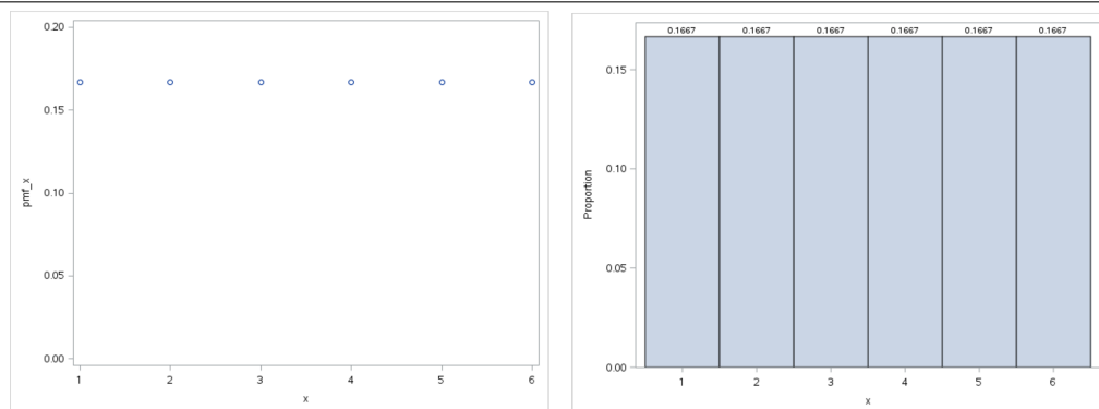
Figure 7.2: Uniform distribution on 1,2,3,4,5,6 – p.m.f. and probability histogram
