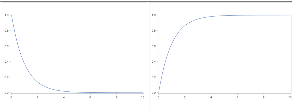
Figure 8.11: The p.d.f. and c.d.f. of the exponential distribution with mean one
