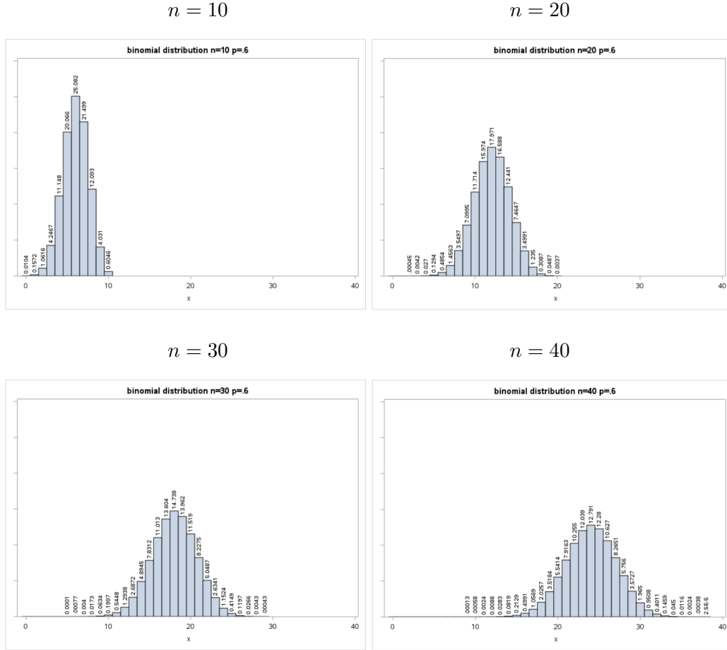
Figure 7.4: Binomial distributions for p=.6 and n=10,20,30,40
