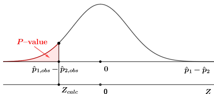
Figure 10.7: P-value for H_1: p_1 less than p_2
