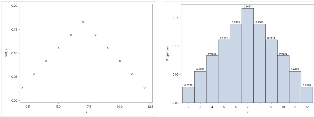
Figure 7.3: Distribution of sum on two tosses of a fair die – p.m.f. and probability histogram (Triangular distribution on 2,3,4,5,6,7,8,9,10,11,12)
