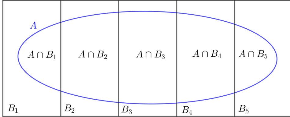
Figure 6.1: The law of total probability
