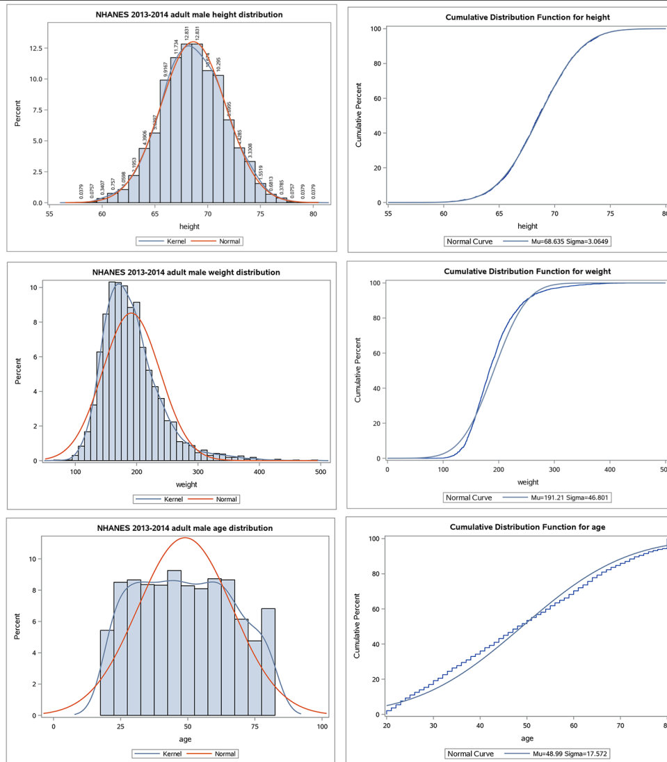
Figure 8.9: NHANES 2013–2014 height, weight, and age distributions for males
