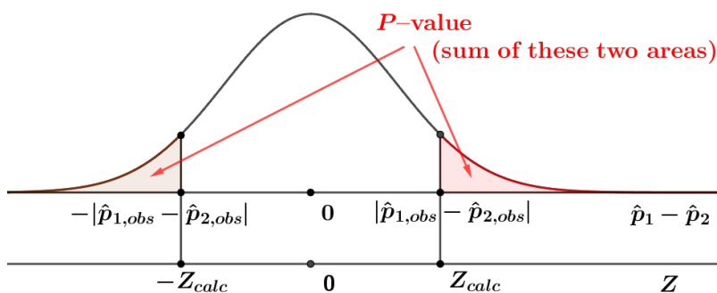
Figure 10.8: P-value for H_1: p_1 not equal to p_2
