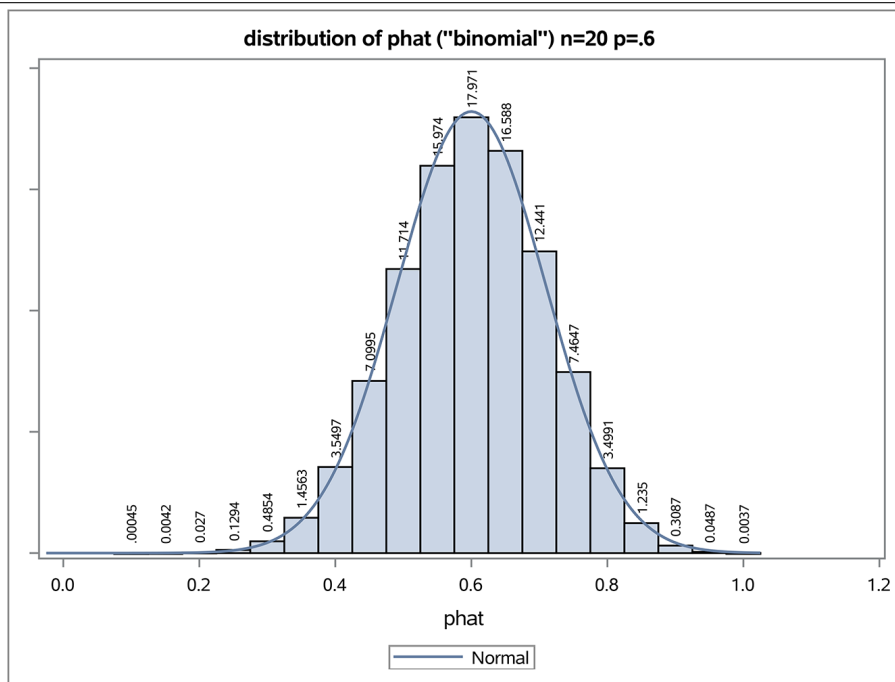
Figure 9.4: Sampling distribution of \hat{p} with normal approximation for n = 20 and p = .6
