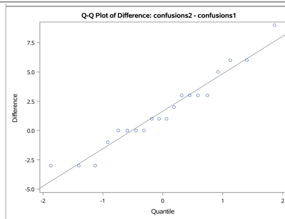
Figure 11.11: Homophone Confusions Example QQ-plot
