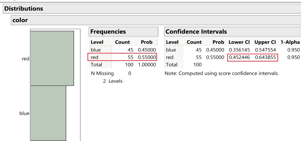
Figure 9.8: JMP output (and commands) for the Wilson 95% confidence interval for the box of balls example
