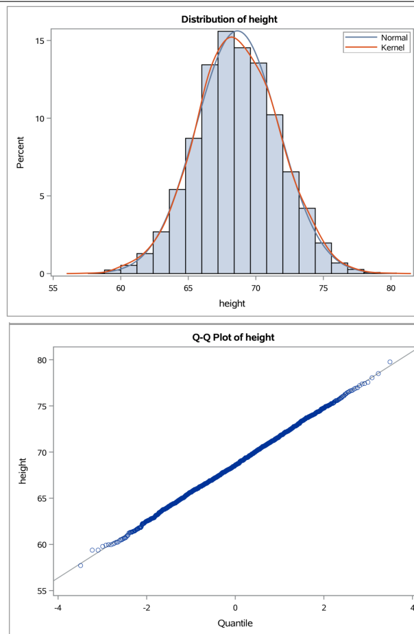
Figure 11.5: NHANES 2013–2014 Height Data for Adult Men
