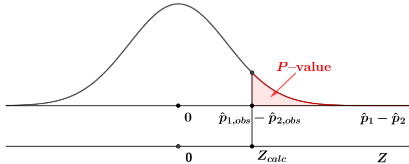
Figure 10.6: P-value for H_1: p_1 greater than p_2
