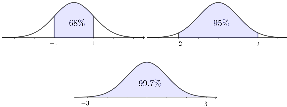
Figure 2.13: 68, 95, 99.7 percent rule graphs
