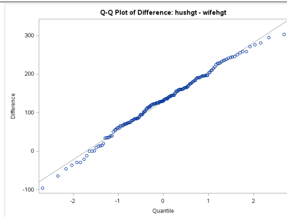
Figure 11.7: Couple height Difference QQ-plot
