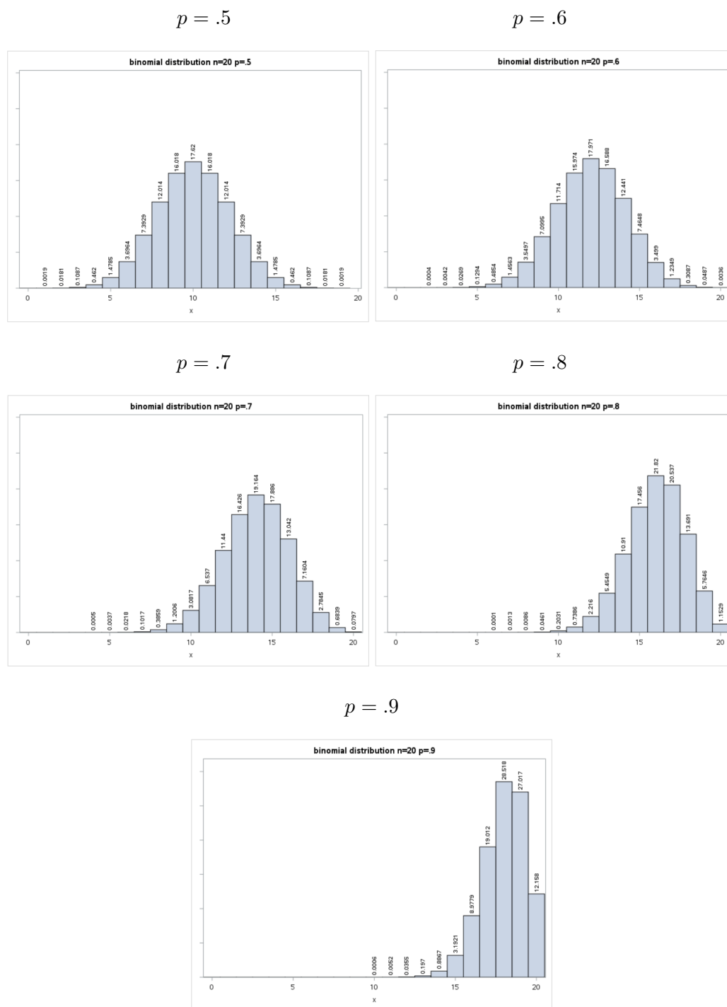
Figure 7.5: Binomial distributions for n=20 and p=.5, .6, .7, .8, .9
