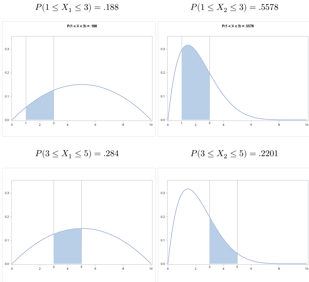
Figure 8.3: Continuous distributions – probability as area
