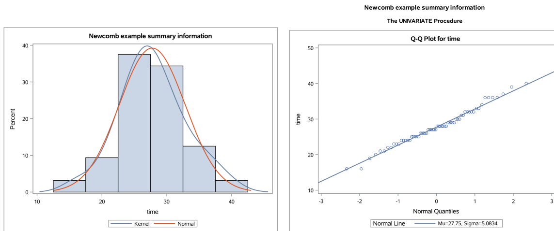
Figure 11.14: Newcomb's Time Data Histogram and QQ-plot
