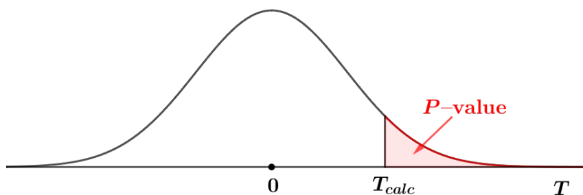
Figure 12.4: P-value for H_1: \mu_1 greater than \mu_2 .
