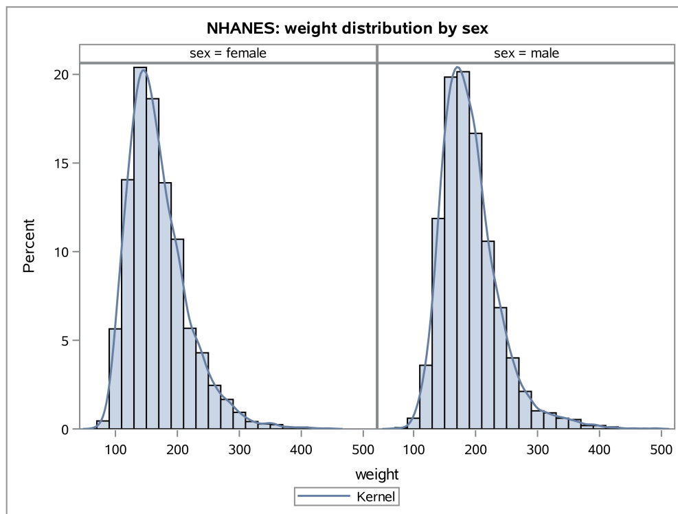
Figure 2.5: NHANES 2013–2014 adult weight distribution histograms
