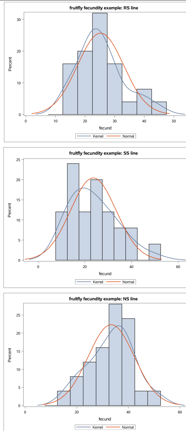
Figure 12.13: Histogram for fecundity by genetic line.
