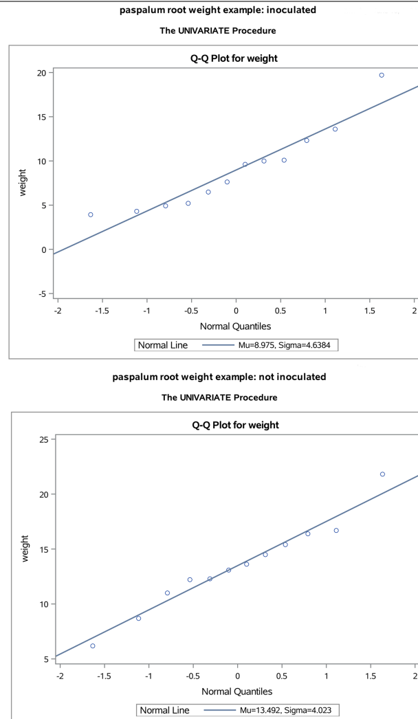
Figure 12.10: QQ plots for paspalum root weight.
