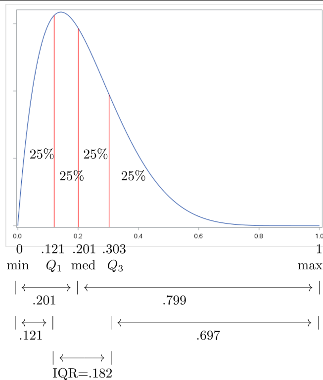
Figure 2.7: Mound shaped, single peak, skewed right distribution
