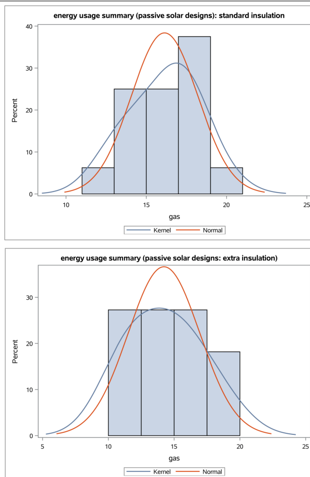
Figure 12.6: Histograms for gas consumption for houses with standard and extra insulation (passive solar).
