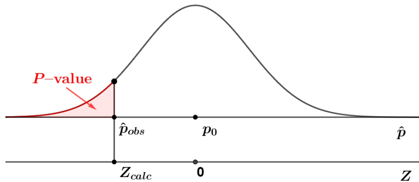
Figure 9.16: P -value for H_0 : p \geq p_0 versus H_1 : p < p_0
