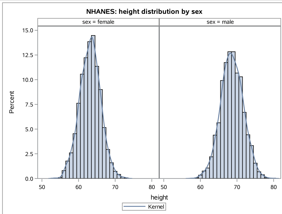
Figure 2.4: NHANES 2013–2014 adult height distribution histograms
