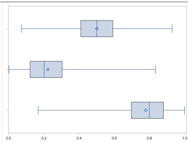
Figure 2.9: Box plots for unimodal mound shaped distributions
