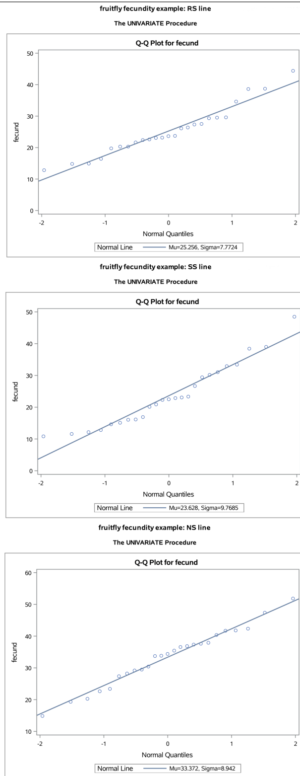
Figure 12.14: QQ plots for fecundity by genetic line.
