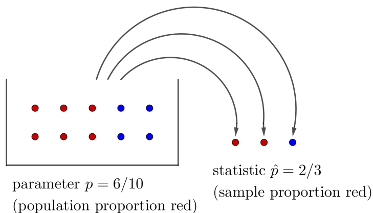
Figure 1.2: Parameter and statistic for a sample from a box of balls
