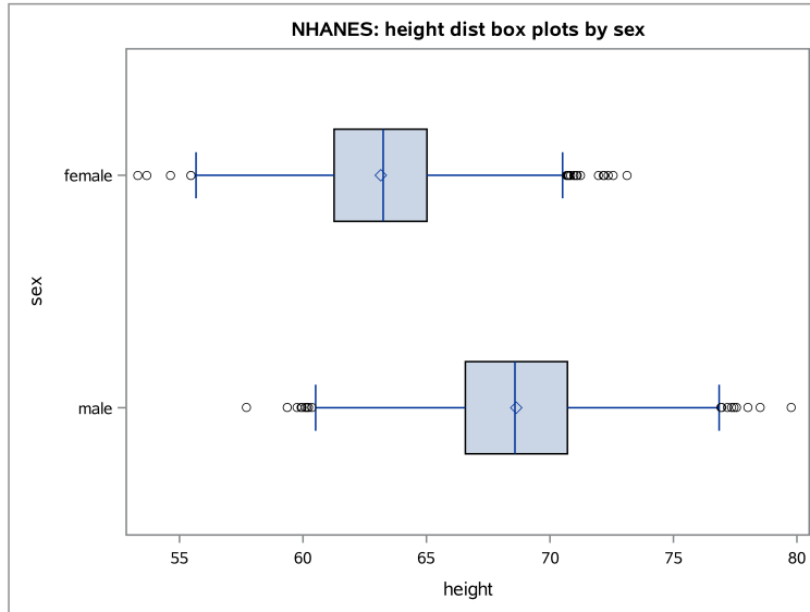
Figure 2.10: NHANES 2013–2014 height distribution boxplots
