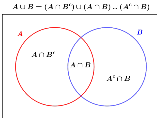
Figure 3.8: Decomposition of the union of A and B
