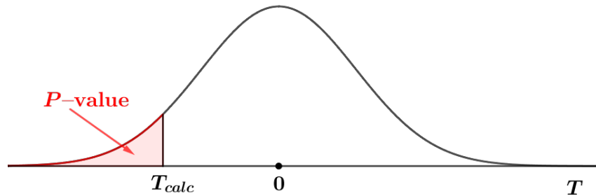
Figure 12.5: P-value for H_1: \mu_1 < \mu_2 .
