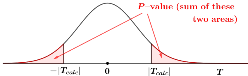
Figure 11.13: P-value for H_1 : mean not equal to \mu_0
