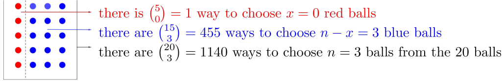
Figure 5.4: Number of choices of balls from a box containing 5 red and 15 blue balls
