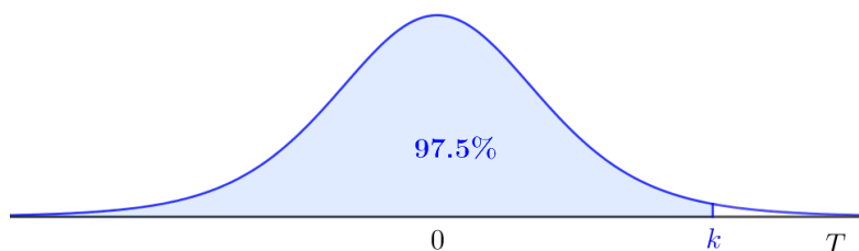
Figure 11.2: Student's t p.d.f. showing 97.5 percentile
