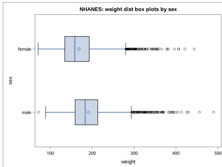
Figure 2.11: NHANES 2013–2014 weight distribution boxplots
