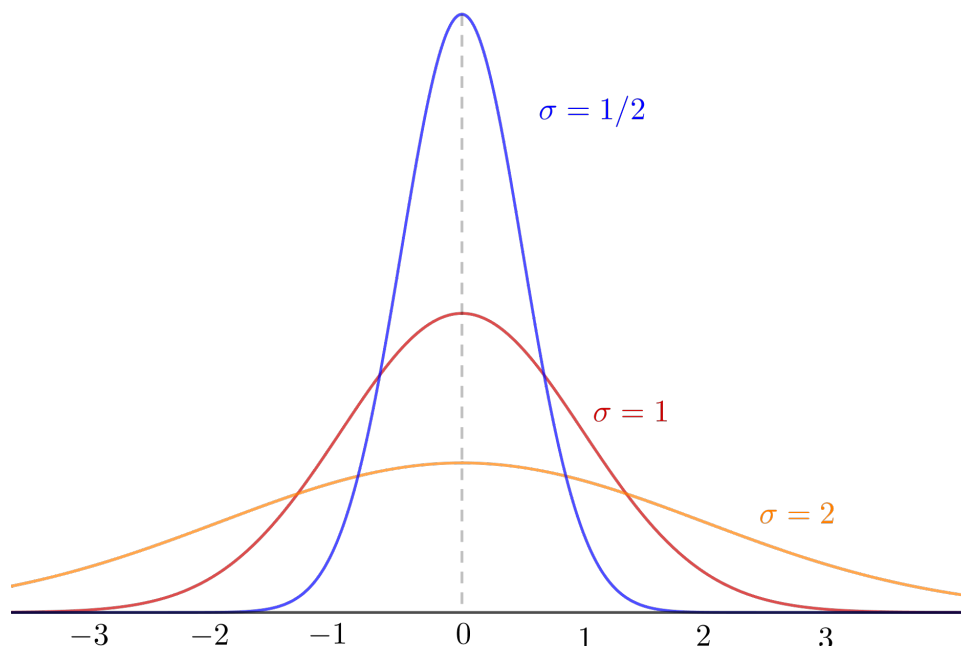
Figure 8.7: Normal distributions with mean zero and standard deviations 1/2 , 1, and 2
