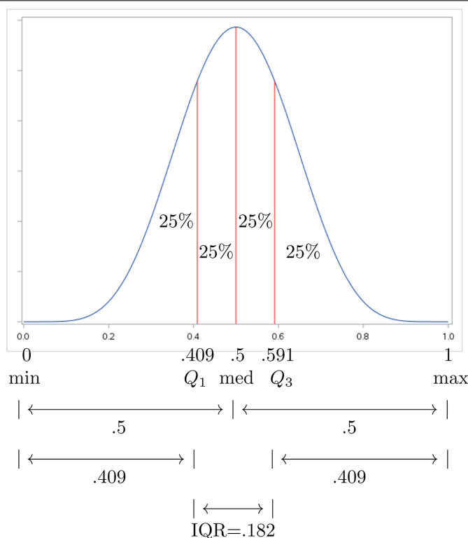
Figure 2.6: Mound shaped, single peak, symmetric distribution
