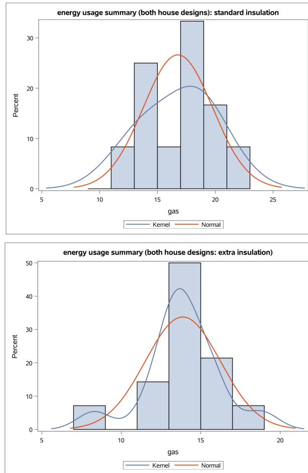
Figure 12.1: Histograms for gas consumption for houses with standard and extra insulation (both designs).
