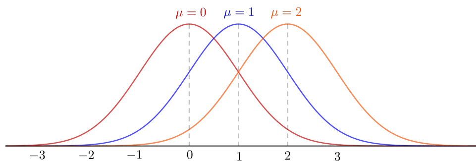
Figure 8.6: Normal distributions with standard deviation one and means of 0, 1, and 2
