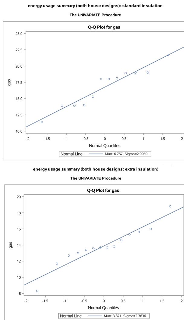
Figure 12.2: QQ plots for gas consumption for houses with standard and extra insulation.
