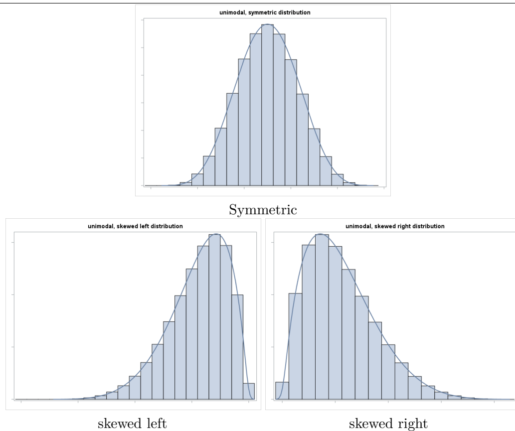
Figure 2.3: Distribution shapes – symmetry and skewness
