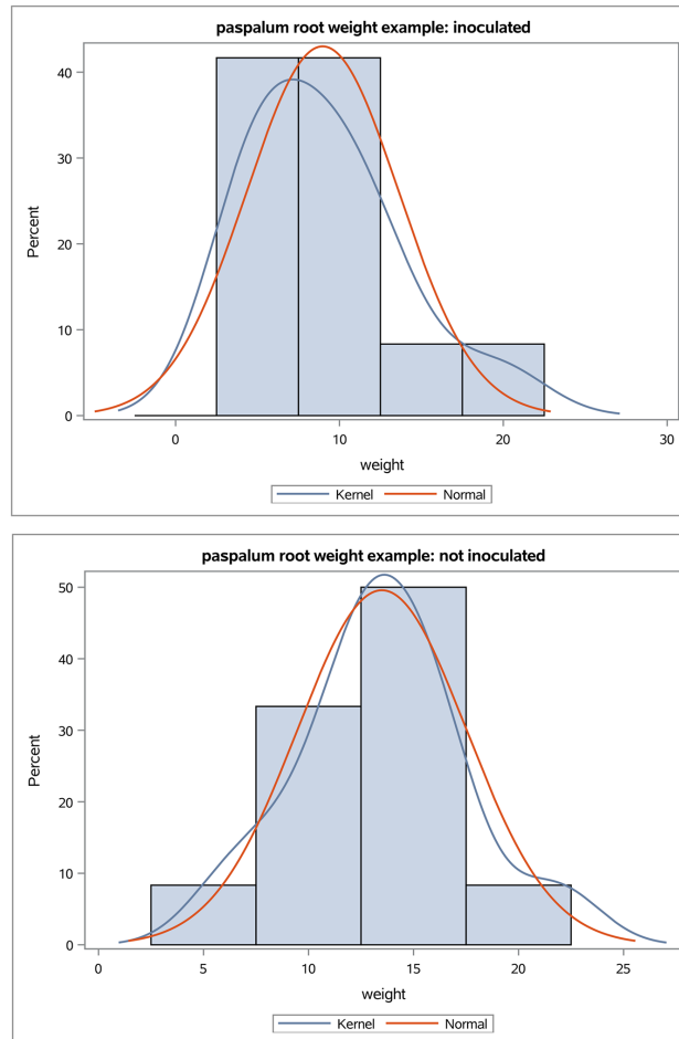
Figure 12.9: Histograms for paspalum root weight.
