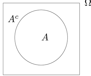
Figure 3.2: An event A and its complement A^c
