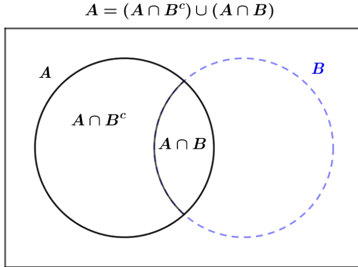
Figure 3.7: Use of event B to decompose event A into two disjoint parts
