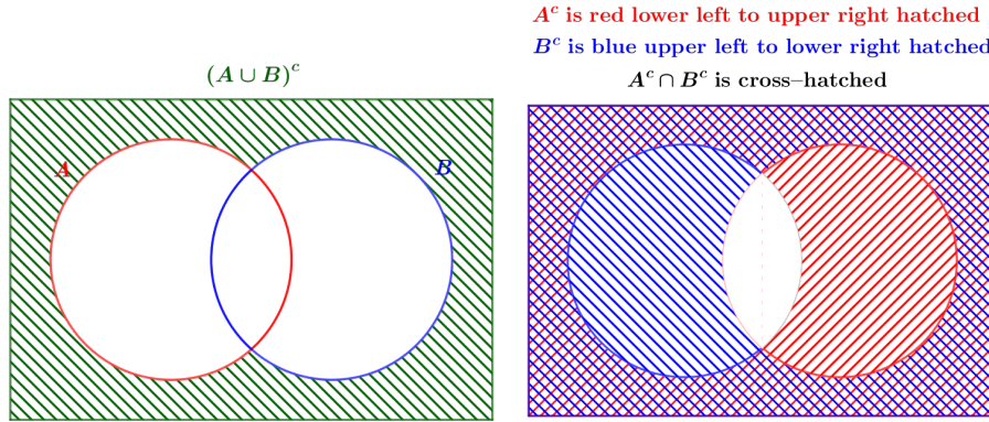
Figure 3.5: Illustration of DeMorgan's law (A \cup B)^c = A^c \cap B^c
