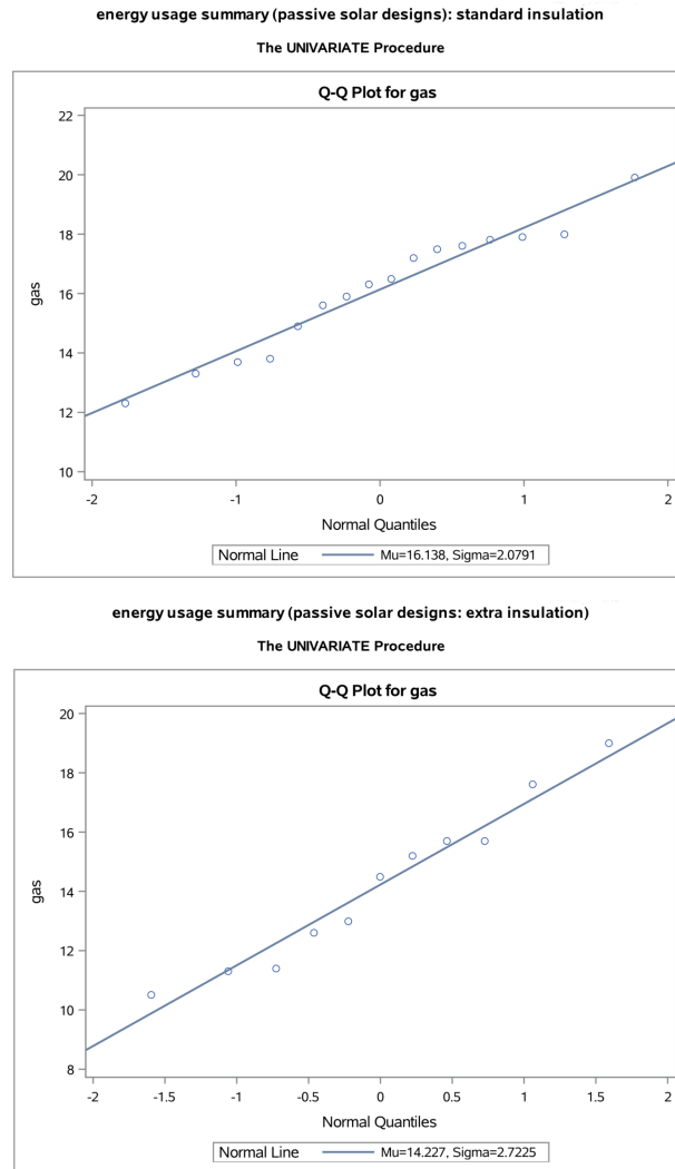
Figure 12.7: QQ plots for gas consumption for houses with standard and extra insulation (passive solar).
