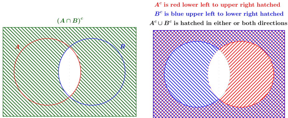
Figure 3.6: Illustration of DeMorgan's law (A \cap B)^c = A^c \cup B^c
