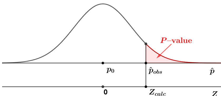
Figure 9.14: P -value for H_0 : p \leq p_0 versus H_1 : p > p_0
