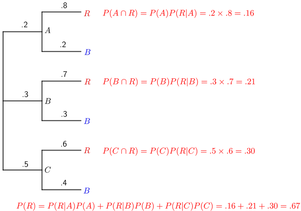
Figure 6.2: A tree diagram for an application of the law of total probability
