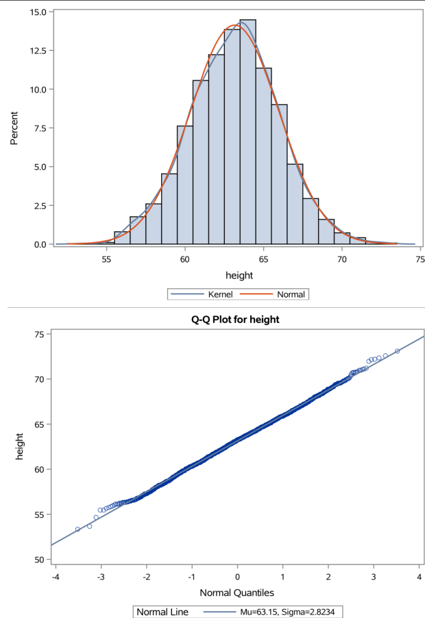
Figure 11.3: NHANES 2013–2014 Height Data for Adult Women
