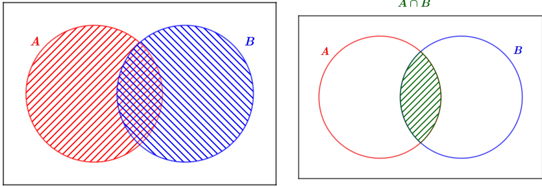
Figure 3.4: The intersection of A and B
