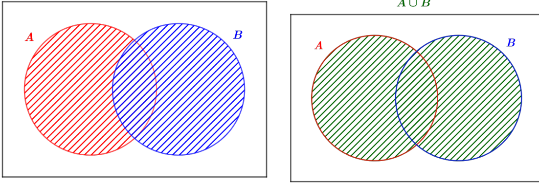
Figure 3.3: The union of A and B
