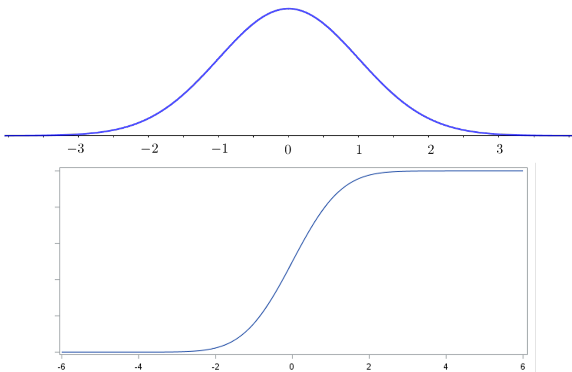
Figure 8.5: The standard normal p.d.f. (density curve) and c.d.f.
