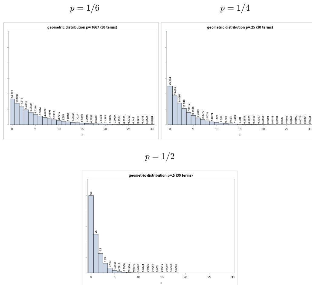
Figure 7.7: Geometric distributions p=1/6, 1/4, 1/2 (first 30 terms)
