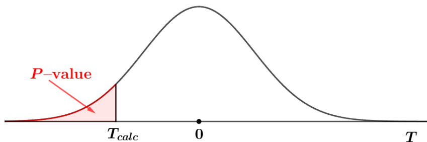
Figure 11.10: P-value for H_1 : mean less than \mu_0
