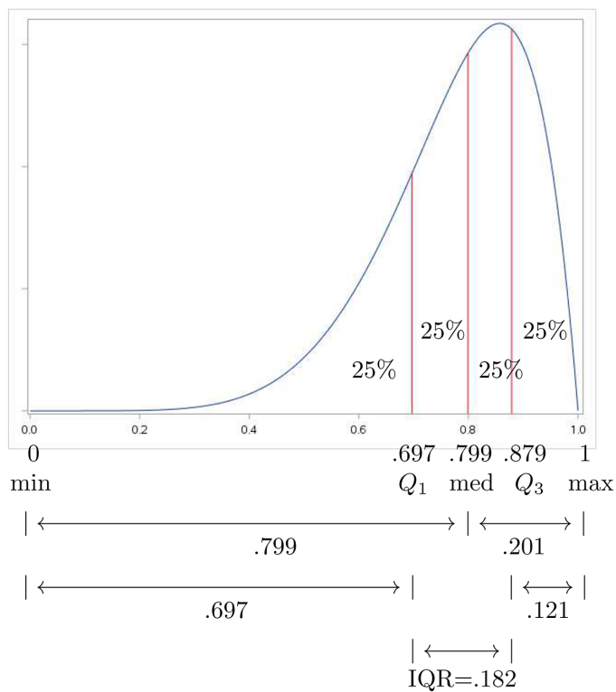
Figure 2.8: Mound shaped, single peak, skewed left distribution
