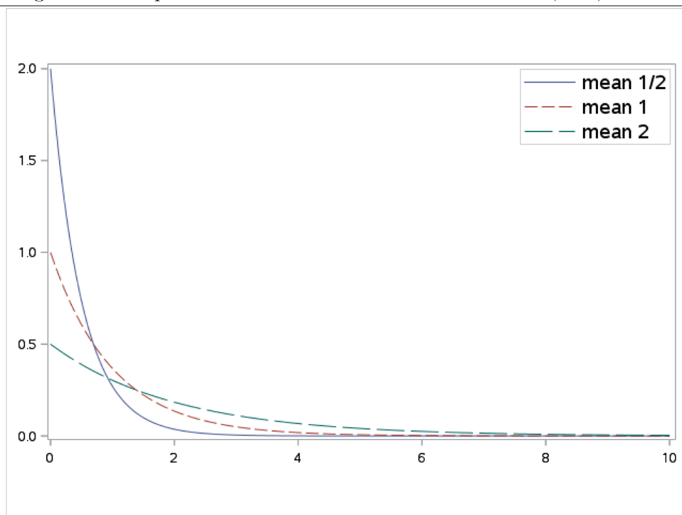
Figure 8.10: Exponential distributions with means one-half, one, and two
