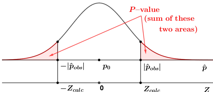
Figure 9.18: P -value for H_0 : p = p_0 versus H_1 : p \neq p_0
