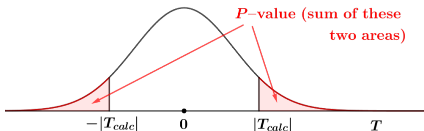
Figure 12.12: P -value for H_1 : \mu_1 not equal to \mu_2 .
