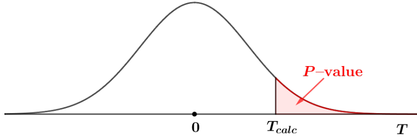
Figure 11.9: P-value for H_1 : mean greater than \mu_0
