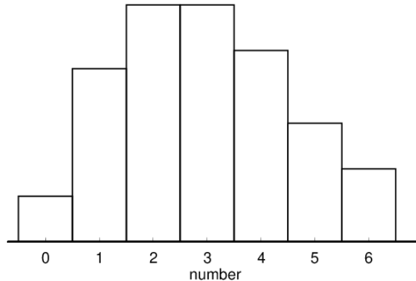
Figure 7.9: Histogram for bacteria counts
