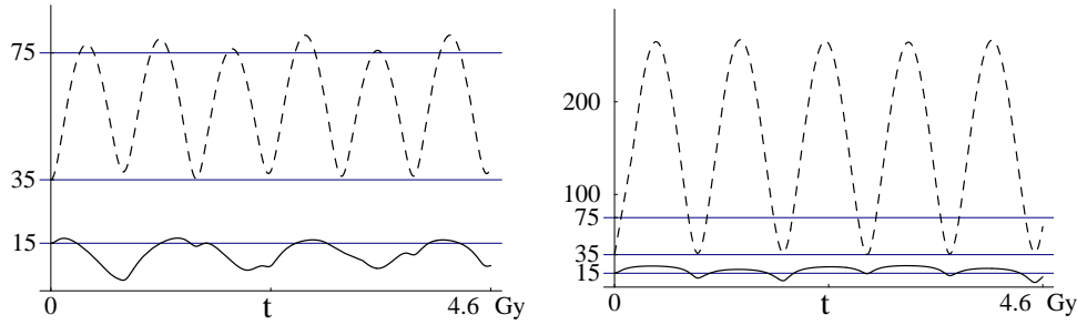
Figure 3. As in figure 2. (left): i_c = 60^\circ , \gamma_c = 5 , \Omega_o = 180^\circ , \omega_o = 180^\circ . (right): i_c = 60^\circ , \gamma_c = 20 , \Omega_o = 180^\circ , \omega_o = 180^\circ .
